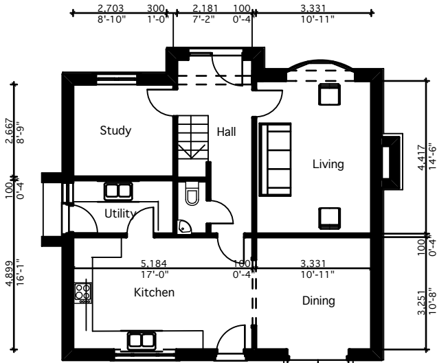
GROUND FLOOR approx area 730sqft
