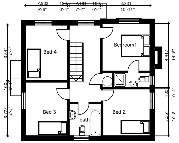
FIRST FLOOR approx area 710sqft
